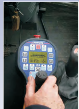
ICS Control
